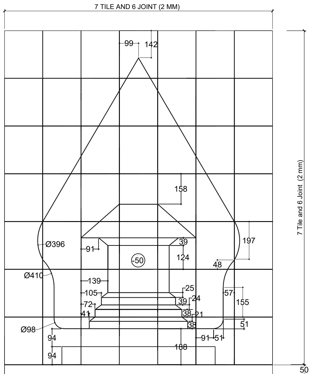
DETAIL UKURAN
