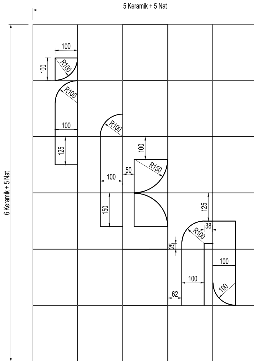
DETAIL MODUL A
