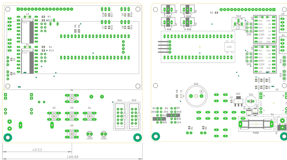
Gambar 1. Board CNC farming robot, bottom and top view
